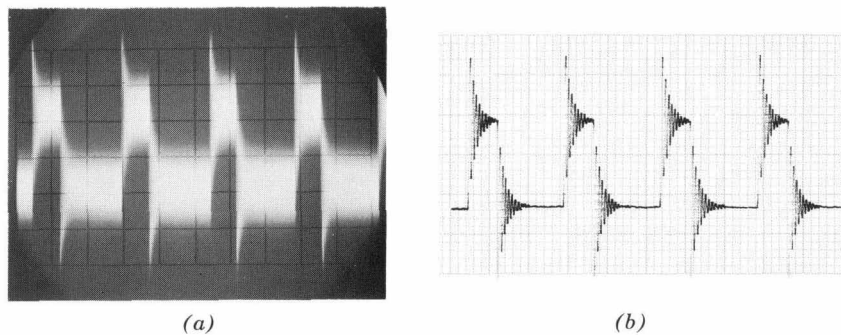
Fig. 5. (a) Oscillogram comparing display of noisy signal with Recorder record (b) in which noise is eliminated. Sweep speed is 2 \mu sec/cm; scope sensitivity is 1 mV/cm. Pulse is 2 mV with 2 mV of noise.
