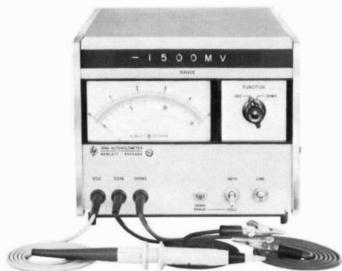
Fig. 2. New -hp- Model 414A Autovoltmeter switches to correct range in less than \frac{1}{3} -second after contact is made. Illuminated display shows range and selected function (volts or ohms). Mirror-backed, taut-band meter has individually-calibrated scales for high accuracy. Separate probes on 4-ft. cables are provided for voltmeter and ohmmeter functions.
