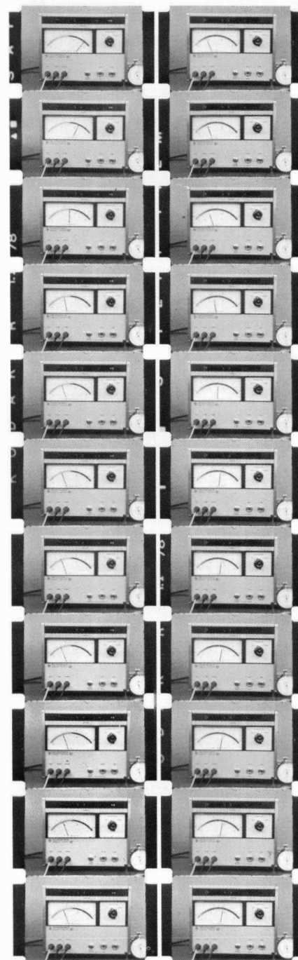
Fig. 3. Speed of response of new Autovoltmeter is shown by film strips photographed at 16 frames per second. In strip at left, input voltage is changed from +14 volts to -15.4 volts following first frame at top of strip. Range change, which requires uprange to 1500V and back down to 50V range, is completed by 10th frame (polarity change requires no switching other than front panel polarity indicator). Meter pointer stabilizes on new reading by 10th frame. Strip at right shows response speed of meter without range change. Following 2nd frame, voltage is switched from +14V to +29.5V. Meter settles on new value by 9th frame, less than one-half second following voltage change.
