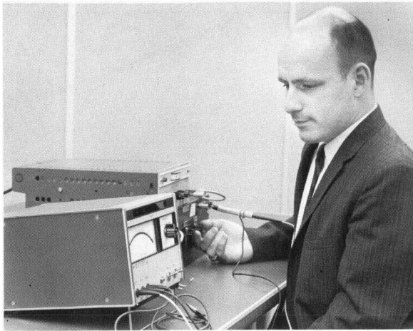
Fig. 6. New autoranging dc volt ohmmeter automatically changes measurement range whenever meter indication exceed 95% of full scale or drops below 25% of full scale. Autoranging speeds measurements in applications such as with dc resistance bridge shown here in which new instrument serves as null detector. Voltmeter switches ranges as required while bridge is brought to balance, thus avoiding overloading or pegging below zero.
