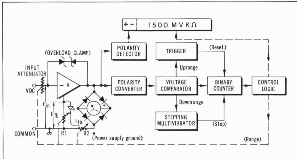
Fig. 4. Block diagram of -hp- Model 414A Autovoltmeter operating in voltmeter mode. Feedback amplifier nulls input voltage E_{in} with voltage E_{fb} across resistor R_1 . Range changing is
